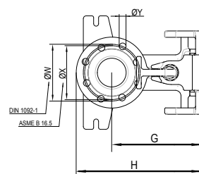
Vista Superior BCS-365
